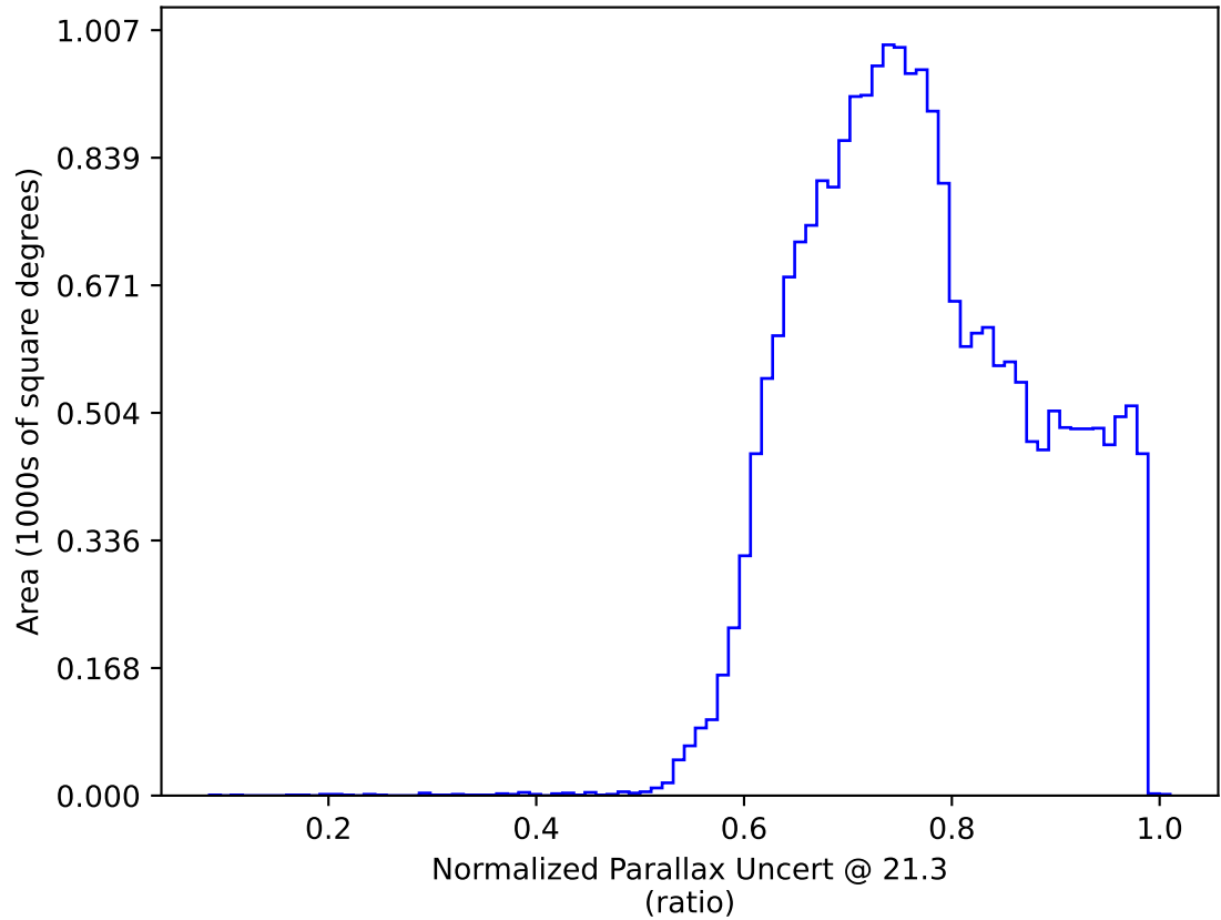
ddf_loaded_half_fl2_v3.4_10yrs All sky y band only: Normalized Parallax Uncert @ 21.3
