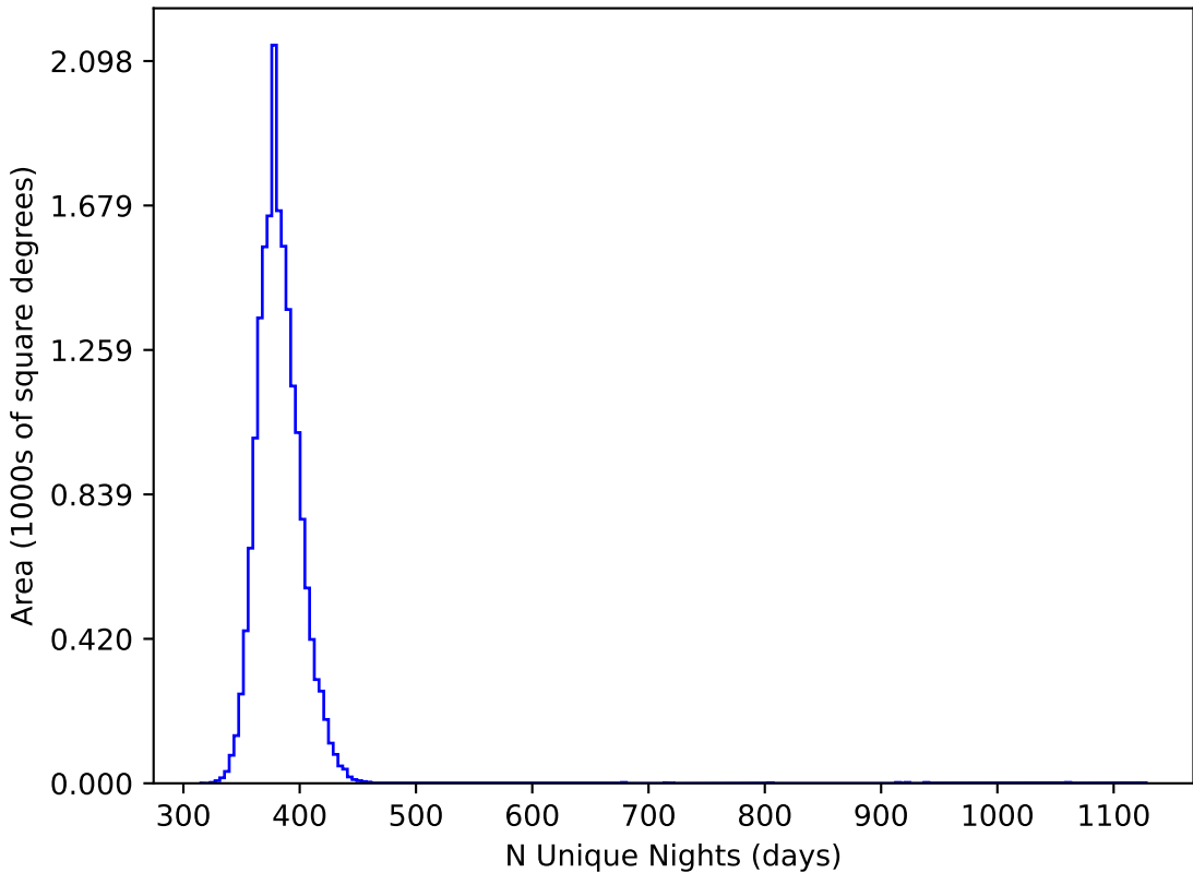
ddf_loaded_half_fl2_v3.4_10yrs WFD all bands: N Unique Nights
