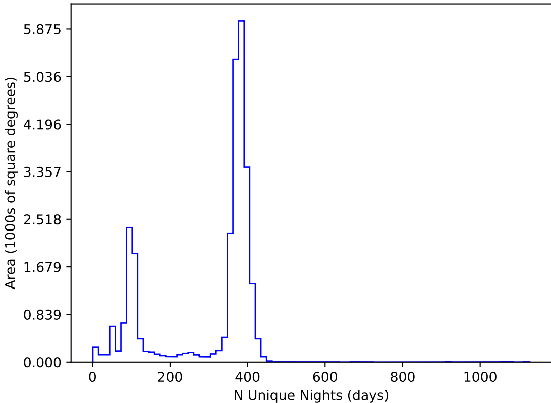
ddf_loaded_half_fl2_v3.4_10yrs All sky all bands: N Unique Nights
