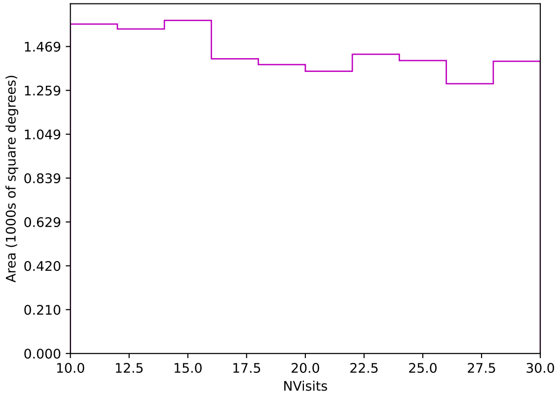
ddf_loaded_half_fl2_v3.4_10yrs Yr 3-4 z band: NVisits
