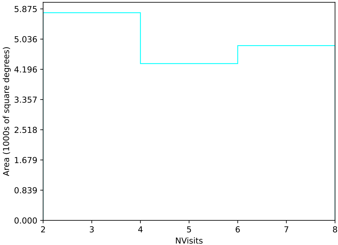
ddf_loaded_half_fl2_v3.4_10yrs Yr 3-4 u band: NVisits
