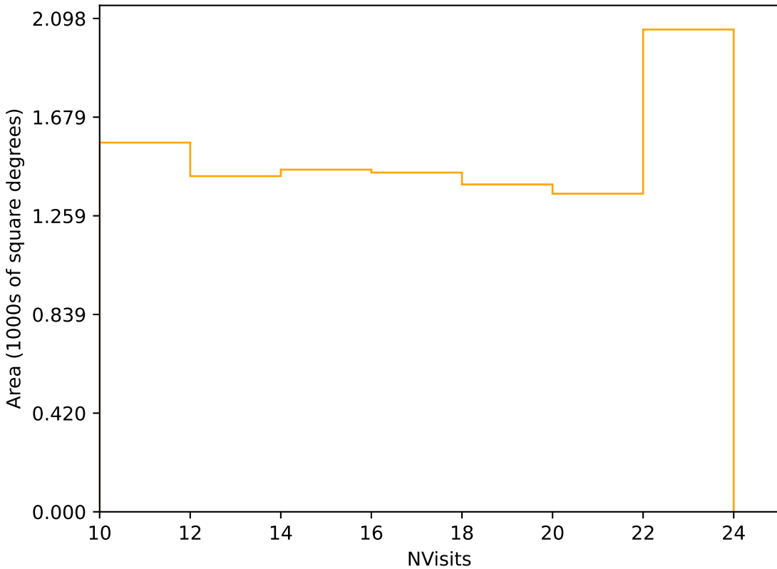
ddf_loaded_half_fl2_v3.4_10yrs Yr 3-4 r band: NVisits
