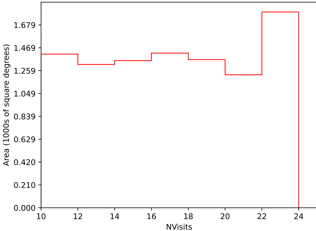
ddf_loaded_half_fl2_v3.4_10yrs Yr 3-4 i band: NVisits
