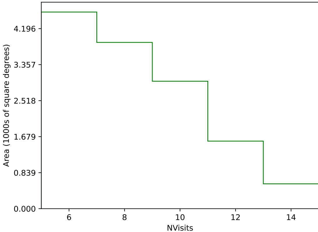
ddf_loaded_half_fl2_v3.4_10yrs Yr 3-4 g band: NVisits
