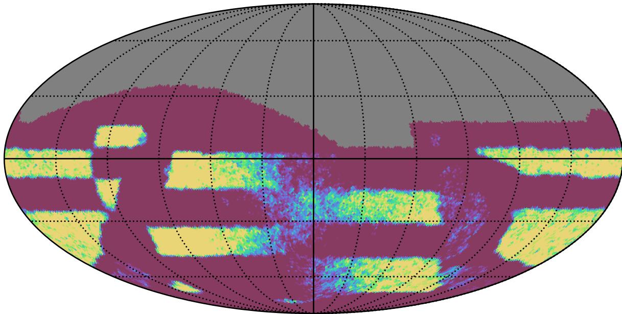
ddf_loaded_half_fl2_v3.4_10yrs Yr 3-4 all bands: NVisits
