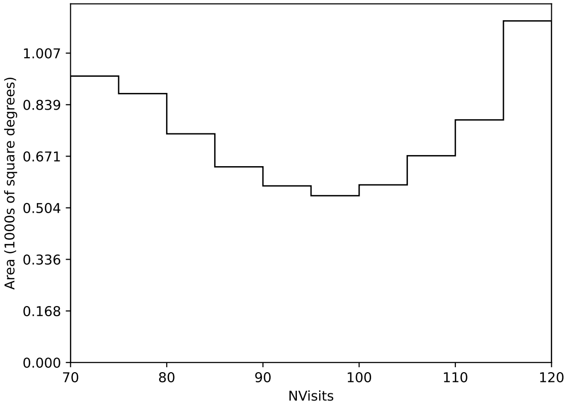
ddf_loaded_half_fl2_v3.4_10yrs Yr 3-4 all bands: NVisits
