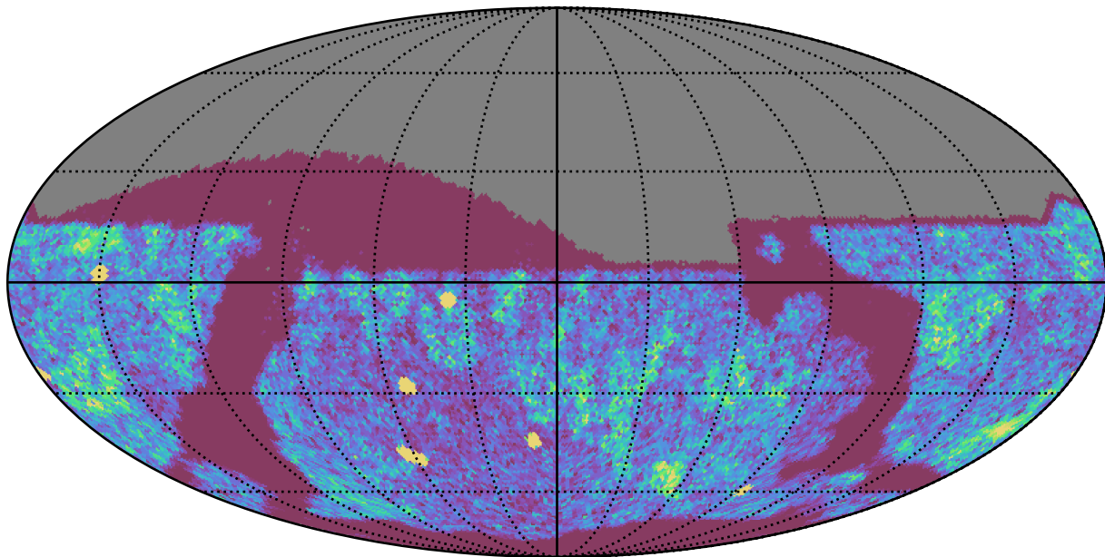
ddf_loaded_half_fl2_v3.4_10yrs Yr 1 z band: NVisits
