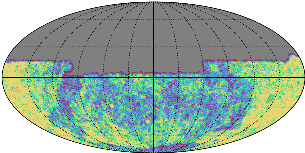
ddf_loaded_half_fl2_v3.4_10yrs Yr 1 u band: NVisits
