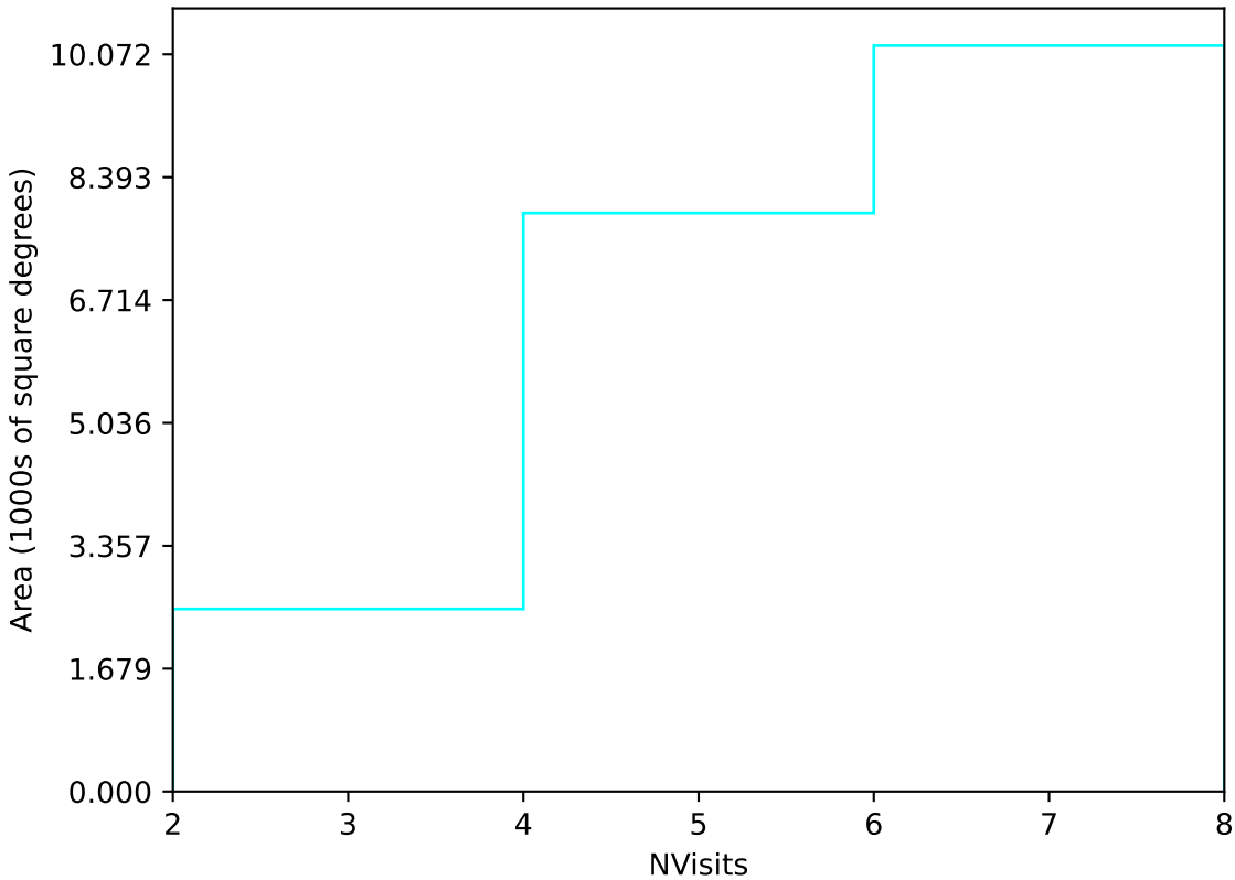
ddf_loaded_half_fl2_v3.4_10yrs Yr 1 u band: NVisits
