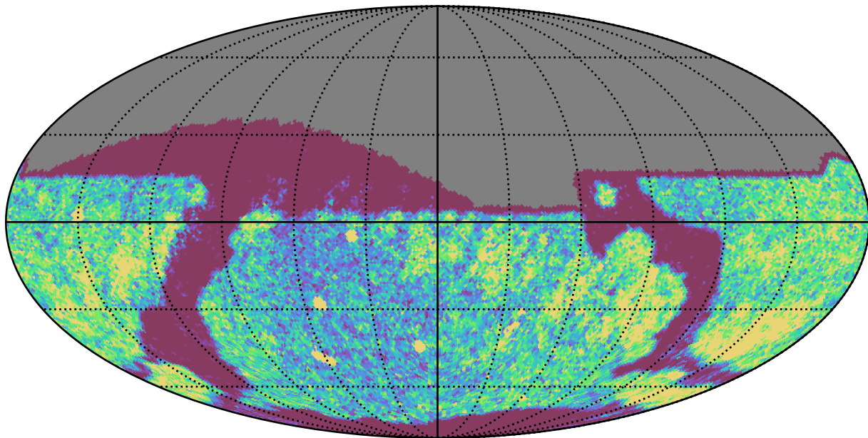
ddf_loaded_half_fl2_v3.4_10yrs Yr 1 r band: NVisits
