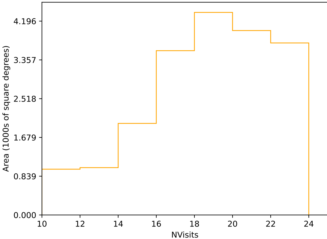
ddf_loaded_half_fl2_v3.4_10yrs Yr 1 r band: NVisits
