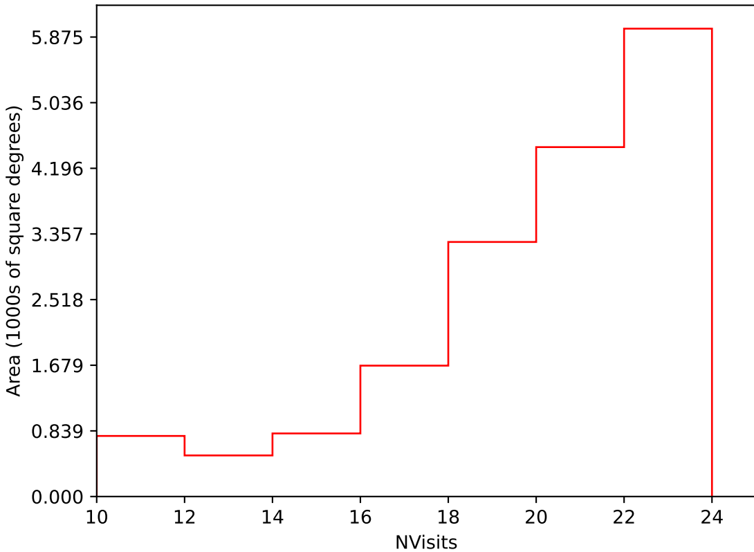
ddf_loaded_half_fl2_v3.4_10yrs Yr 1 i band: NVisits
