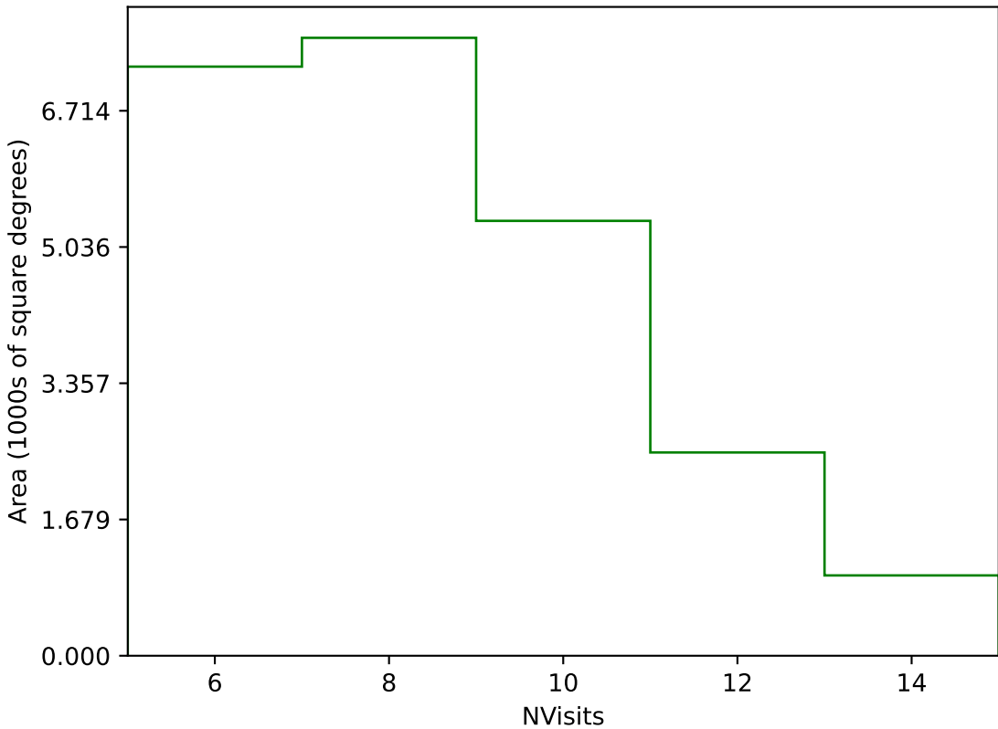
ddf_loaded_half_fl2_v3.4_10yrs Yr 1 g band: NVisits
