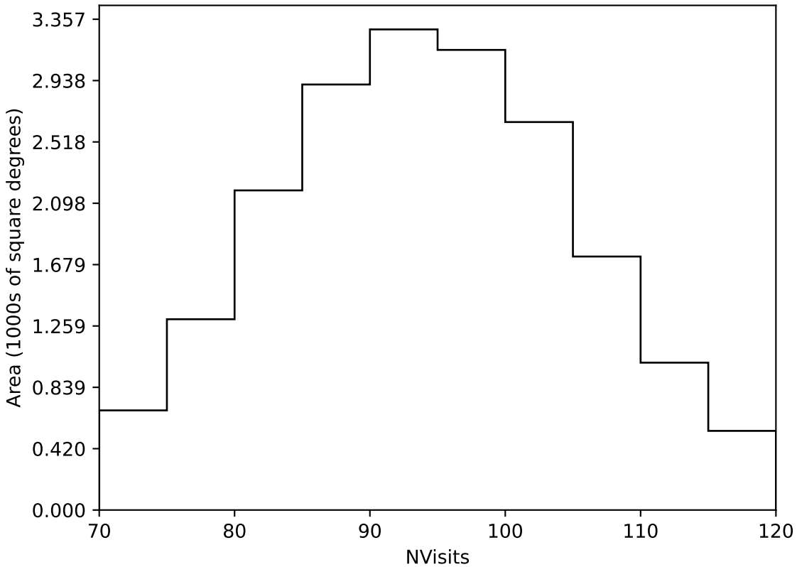
ddf_loaded_half_fl2_v3.4_10yrs Yr 1 all bands: NVisits
