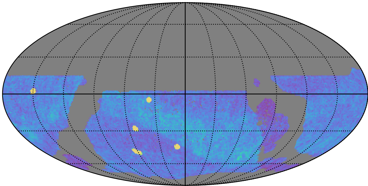
ddf_loaded_half_fl2_v3.4_10yrs WFD z band: NVisits
