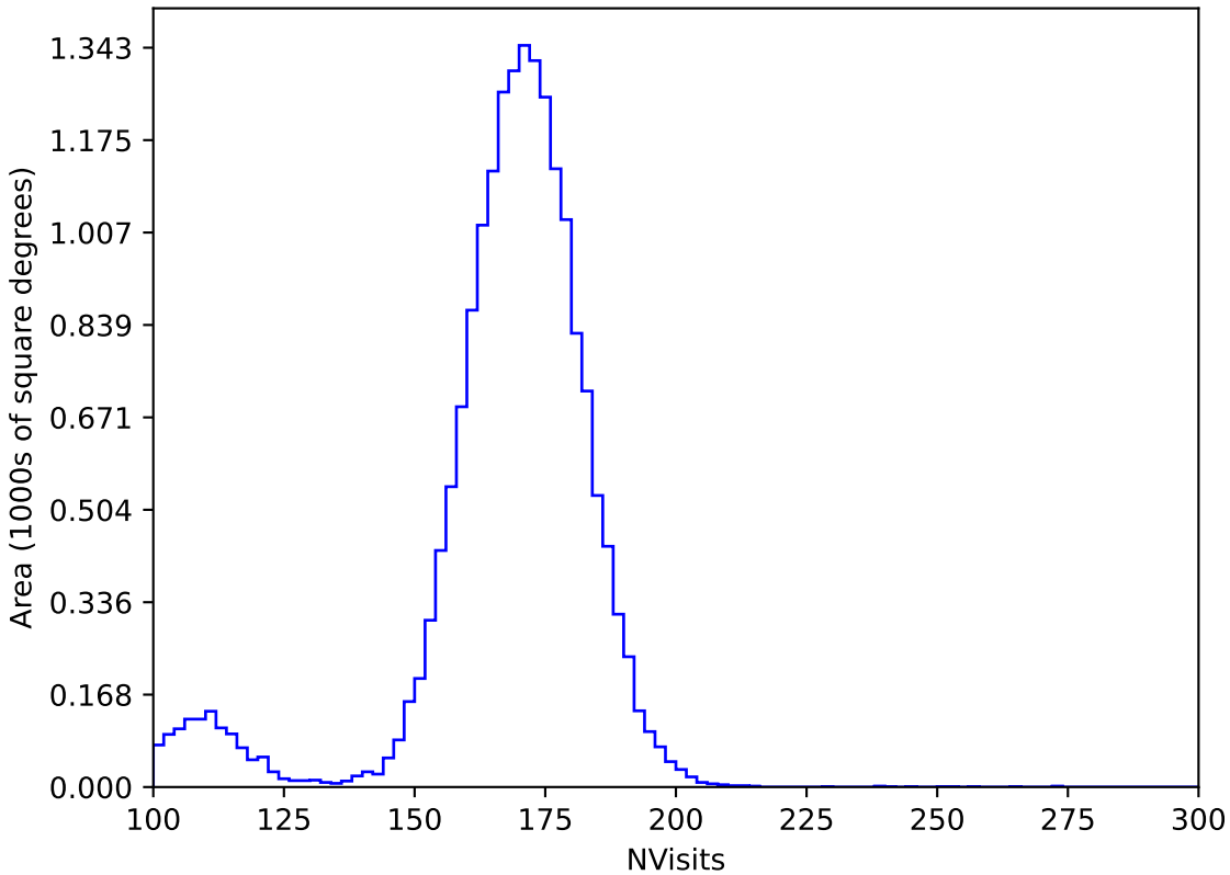
ddf_loaded_half_fl2_v3.4_10yrs WFD y band: NVisits
