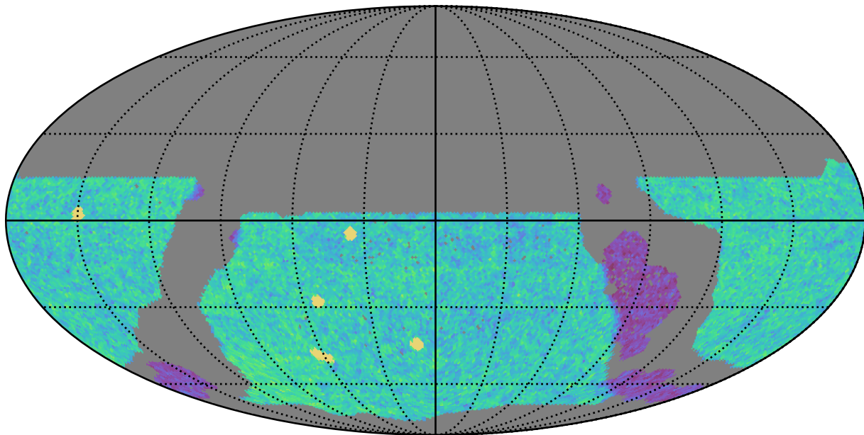
ddf_loaded_half_fl2_v3.4_10yrs WFD u band: NVisits
