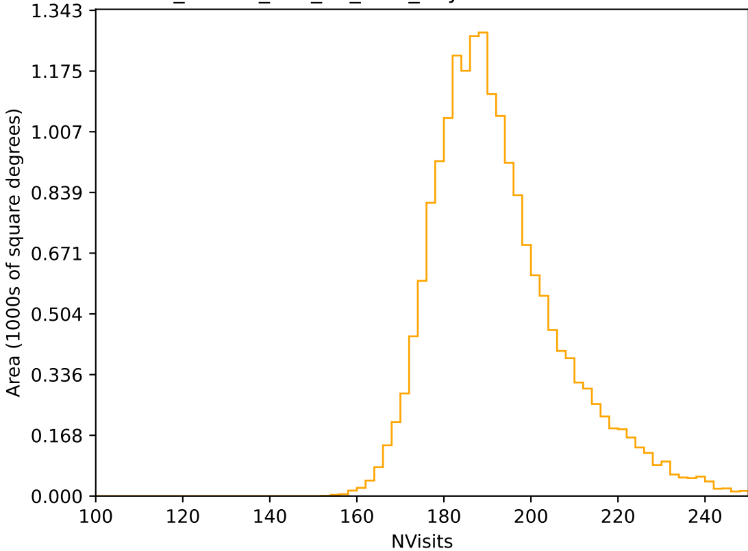
ddf_loaded_half_fl2_v3.4_10yrs WFD r band: NVisits
