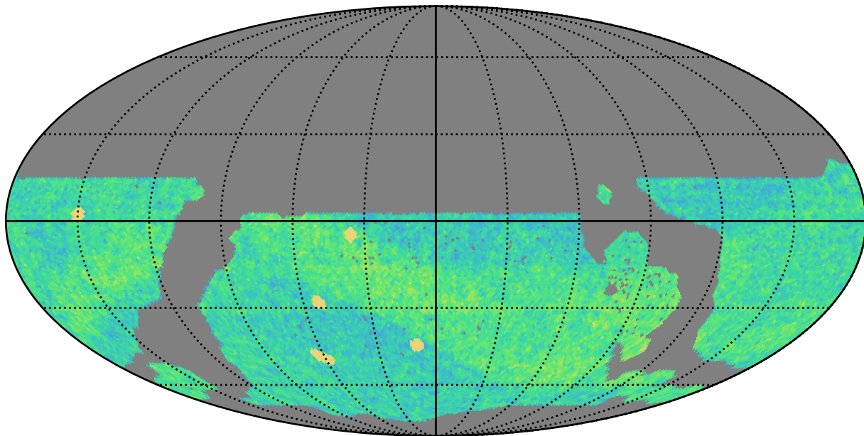
ddf_loaded_half_fl2_v3.4_10yrs WFD i band: NVisits
