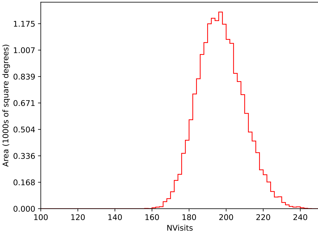
ddf_loaded_half_fl2_v3.4_10yrs WFD i band: NVisits
