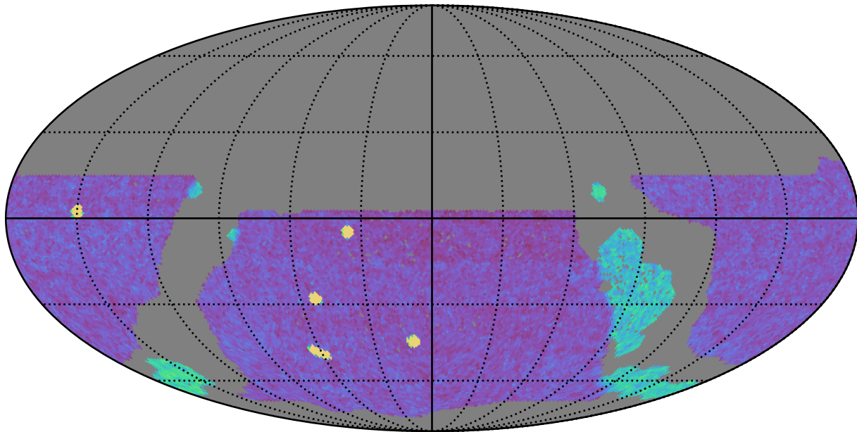
ddf_loaded_half_fl2_v3.4_10yrs WFD g band: NVisits
