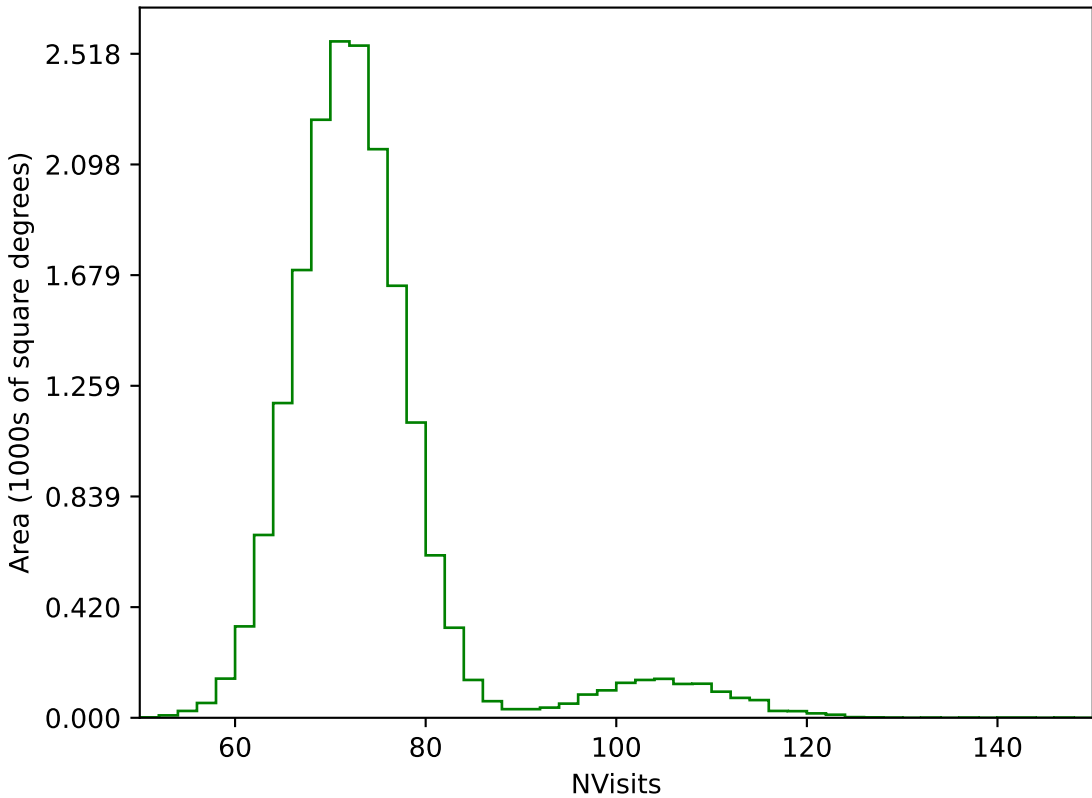
ddf_loaded_half_fl2_v3.4_10yrs WFD g band: NVisits
