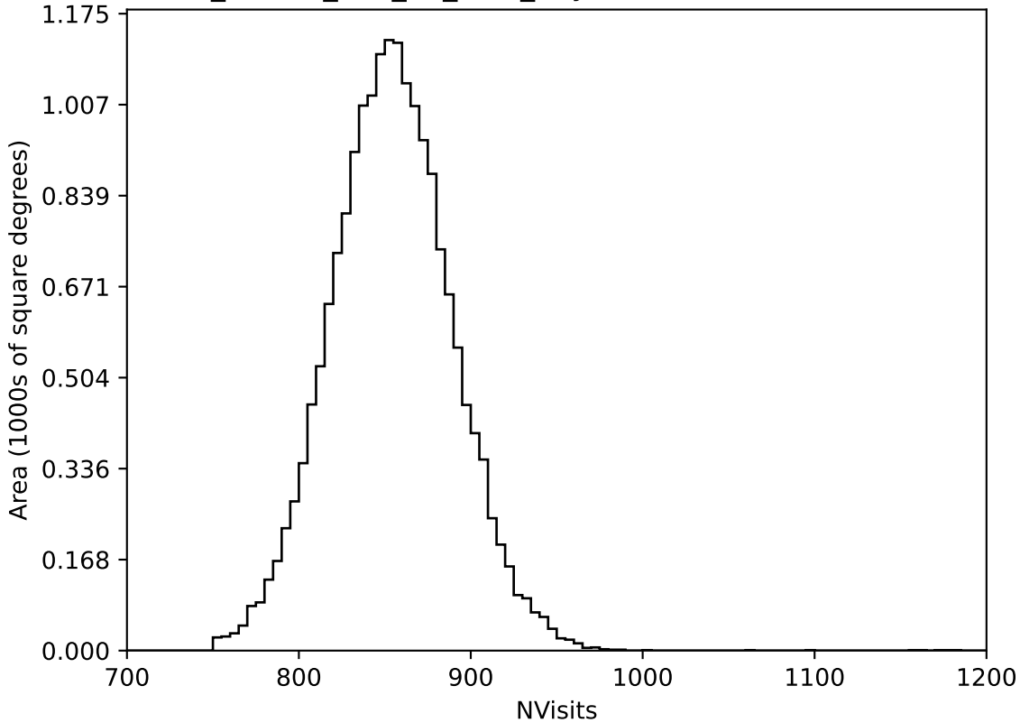
ddf_loaded_half_fl2_v3.4_10yrs WFD all bands: NVisits
