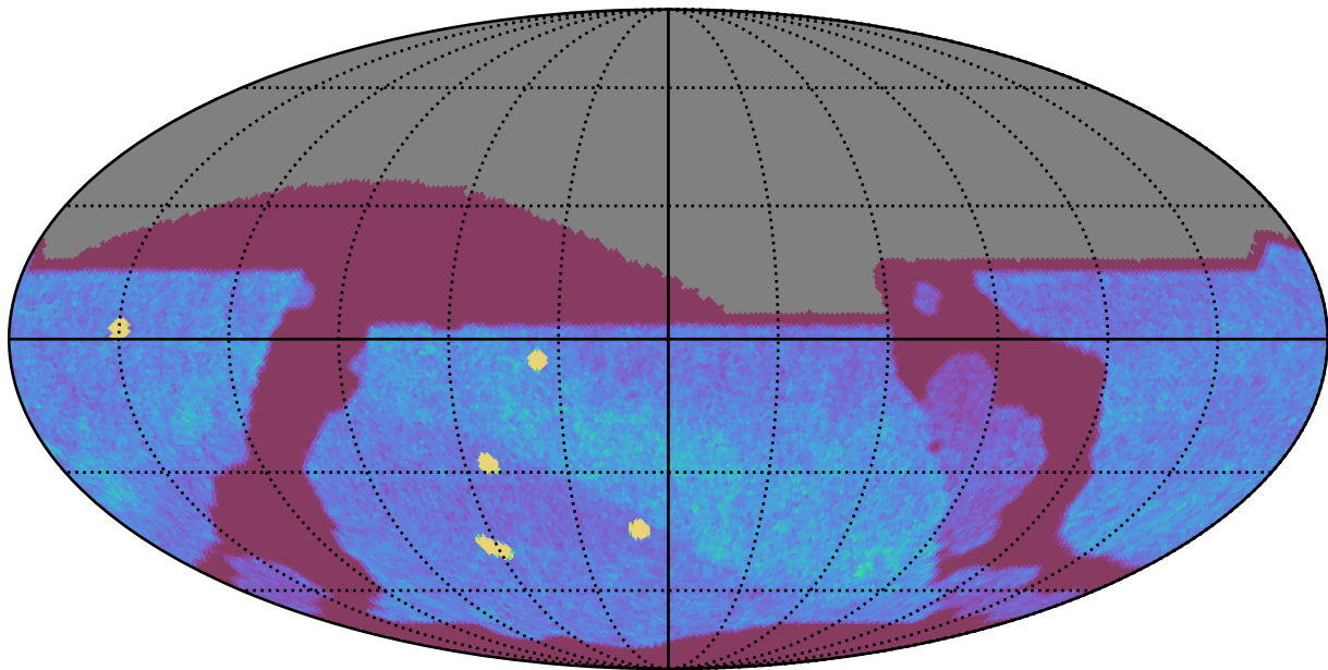
ddf_loaded_half_fl2_v3.4_10yrs All sky z band: NVisits
