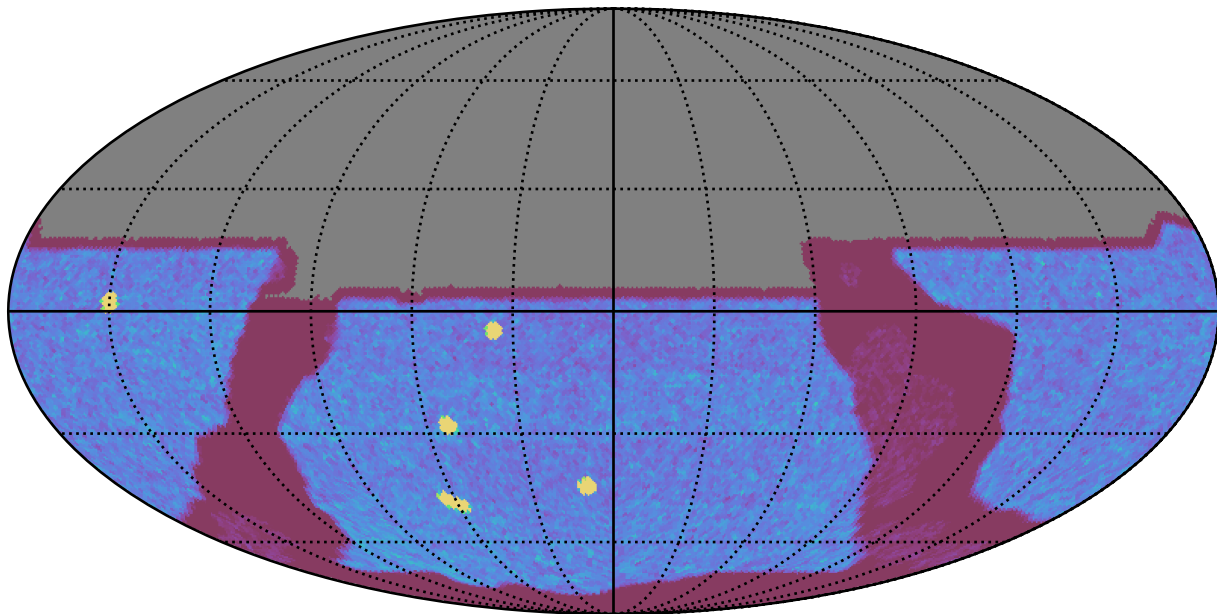
ddf_loaded_half_fl2_v3.4_10yrs All sky y band: NVisits
