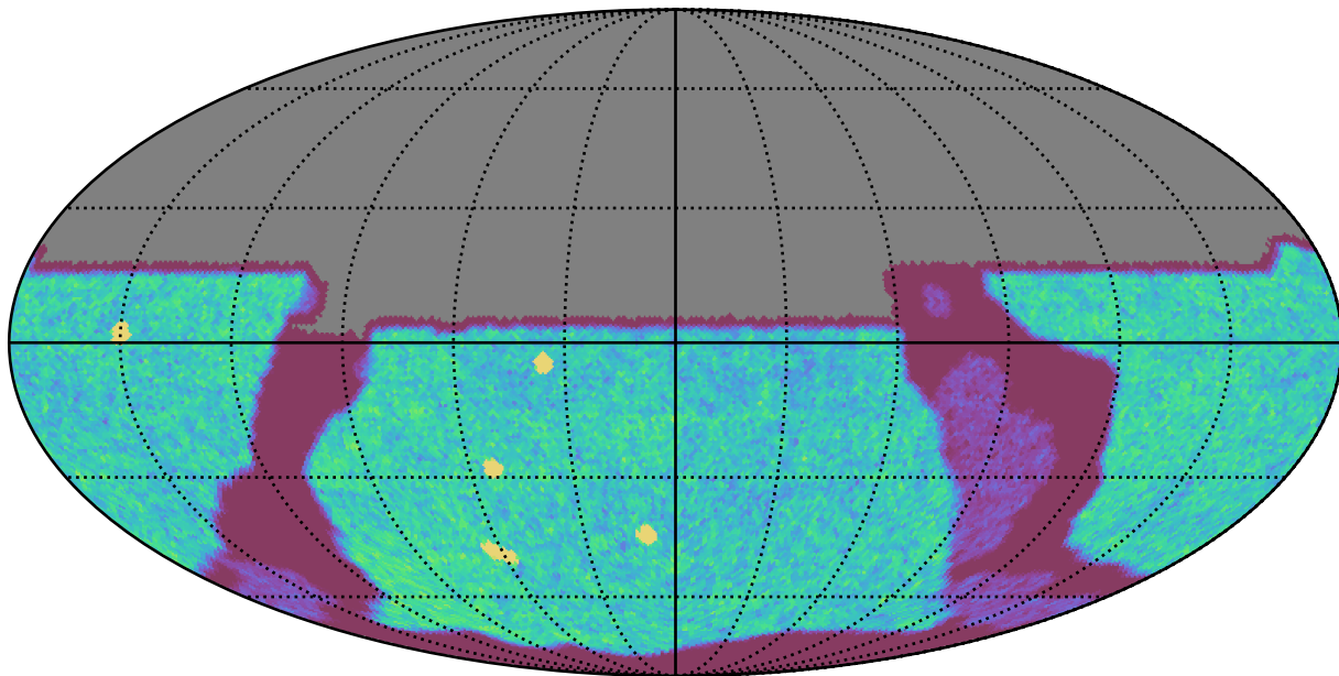
ddf_loaded_half_fl2_v3.4_10yrs All sky u band: NVisits
