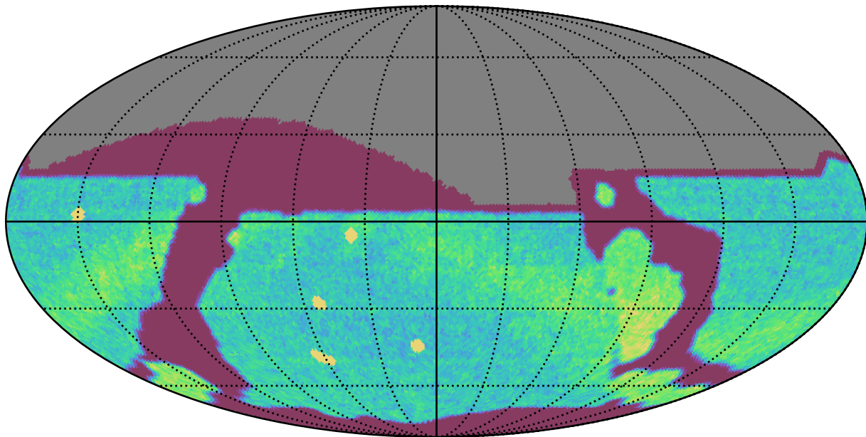
ddf_loaded_half_fl2_v3.4_10yrs All sky r band: NVisits
