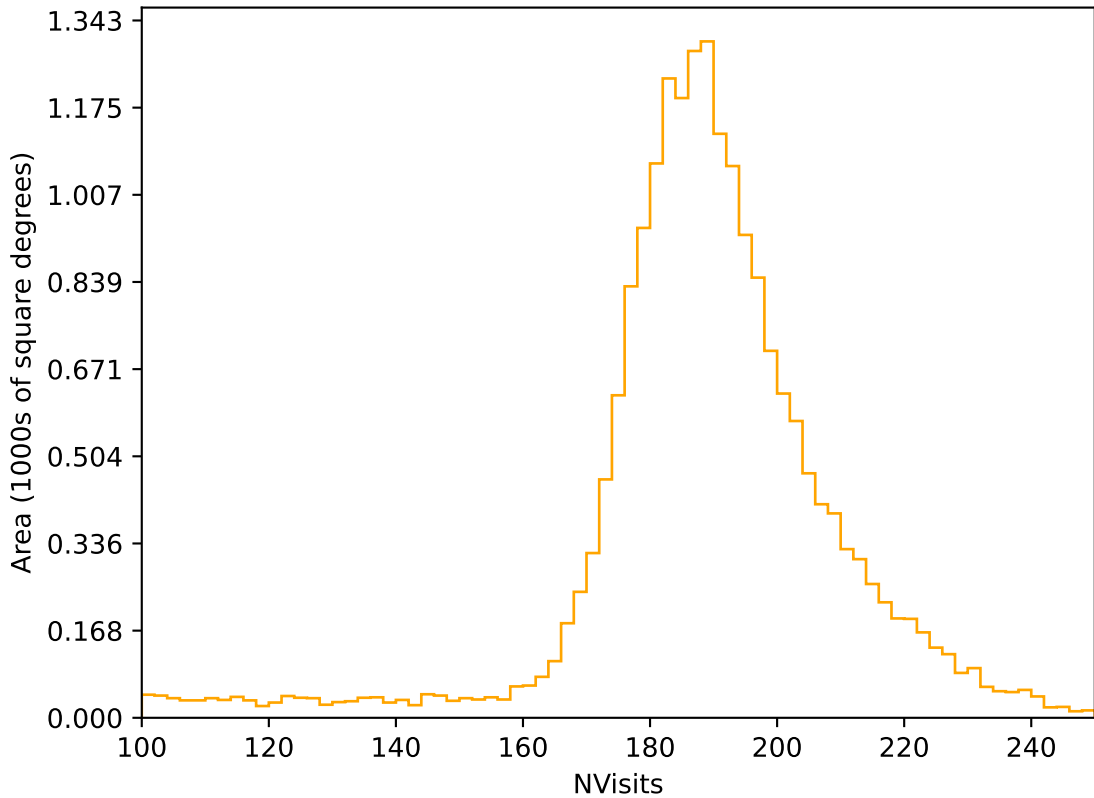
ddf_loaded_half_fl2_v3.4_10yrs All sky r band: NVisits
