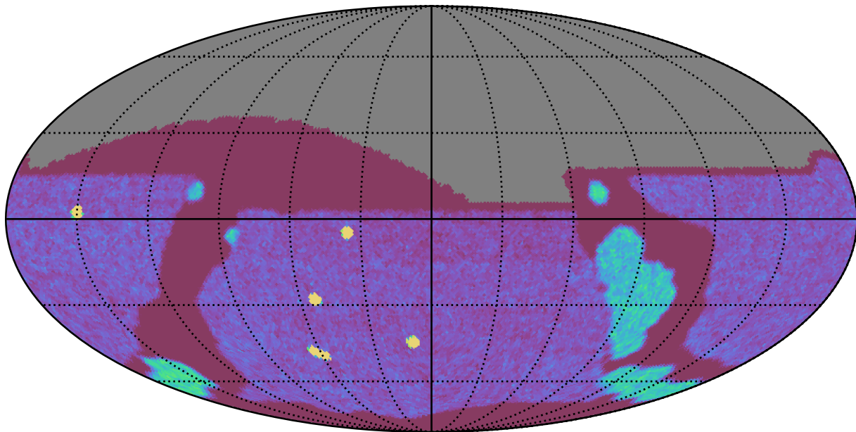
ddf_loaded_half_fl2_v3.4_10yrs All sky g band: NVisits
