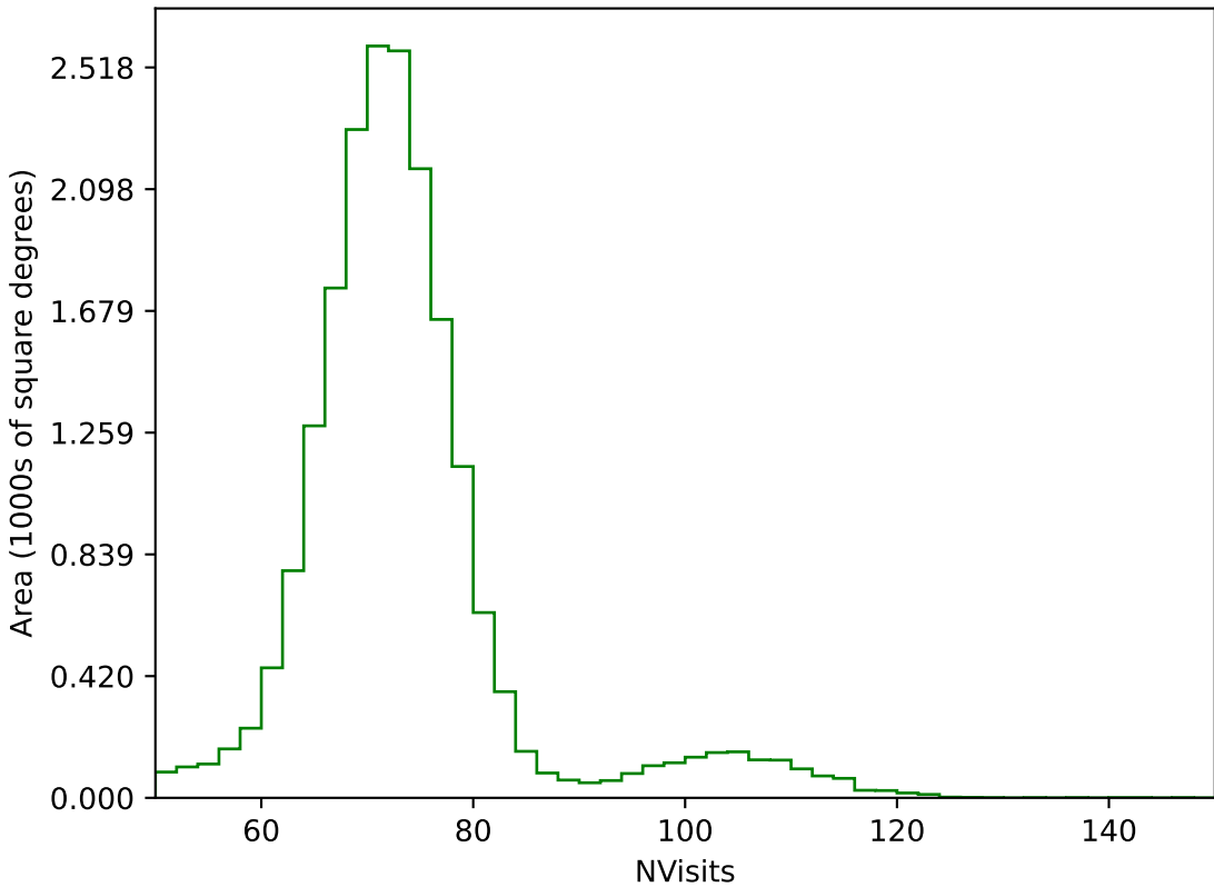
ddf_loaded_half_fl2_v3.4_10yrs All sky g band: NVisits
