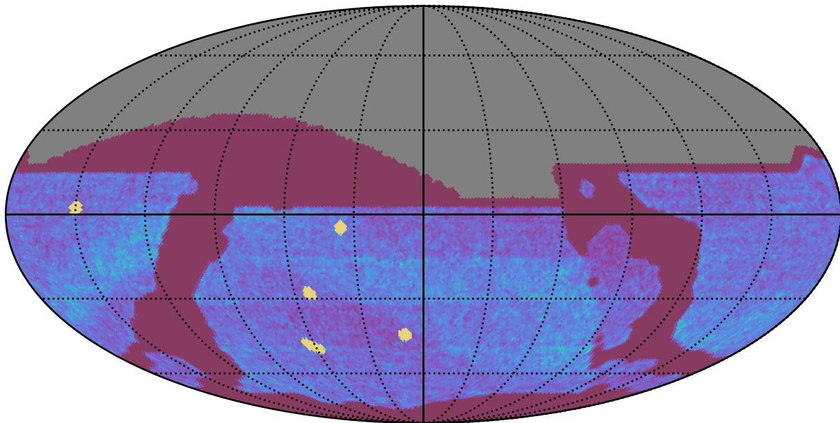
ddf_loaded_half_f12_v3.4_10yrs All sky all bands: NVisits
