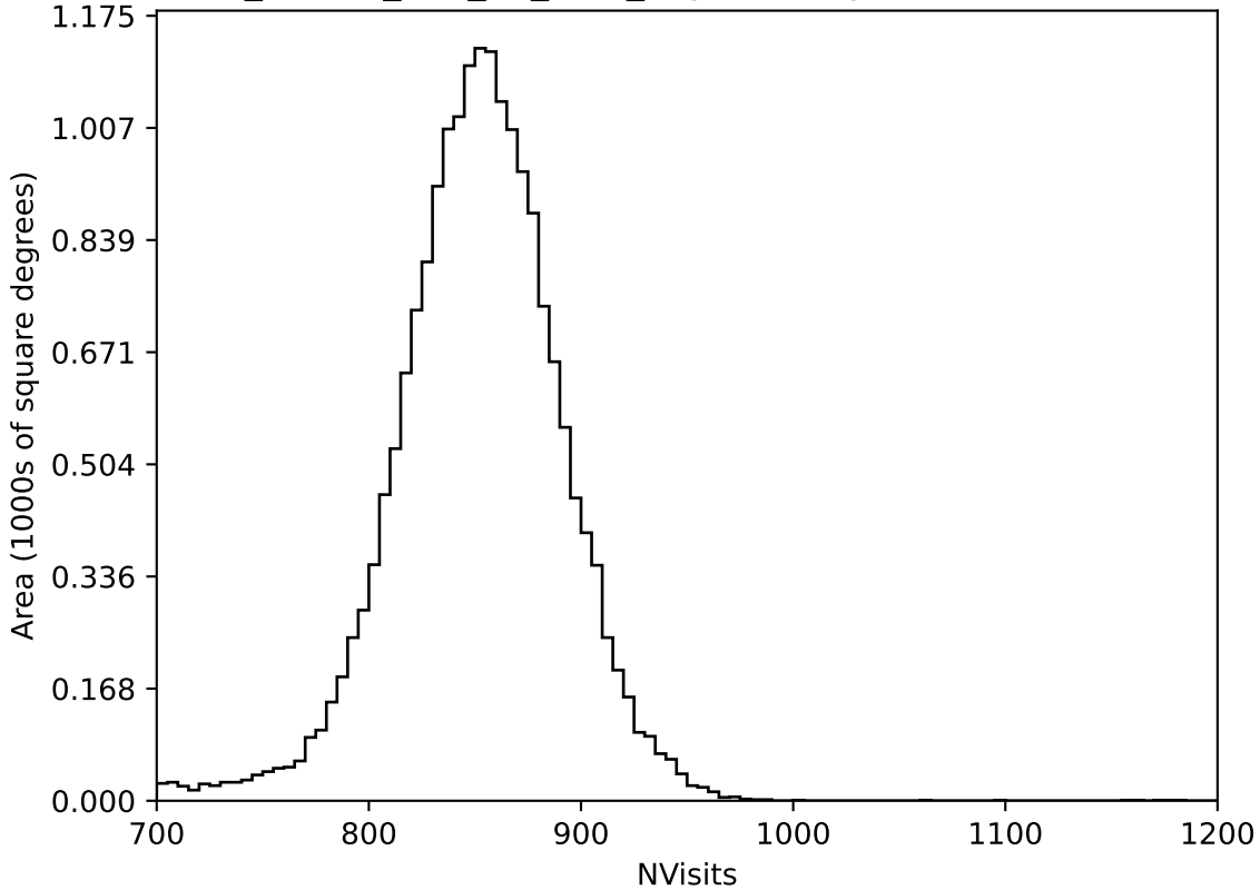
ddf_loaded_half_fl2_v3.4_10yrs All sky all bands: NVisits
