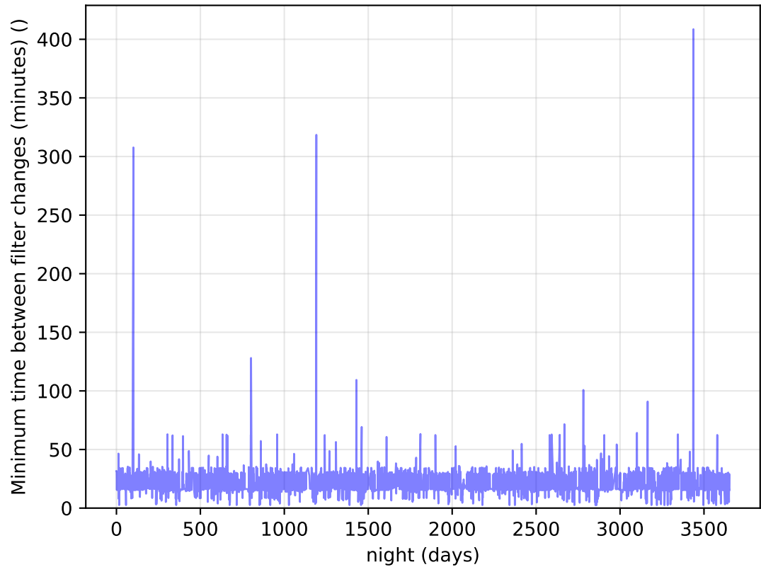
ddf_loaded_half_fl2_v3.4_10yrs Per Night: Minimum time between filter changes (minutes)
