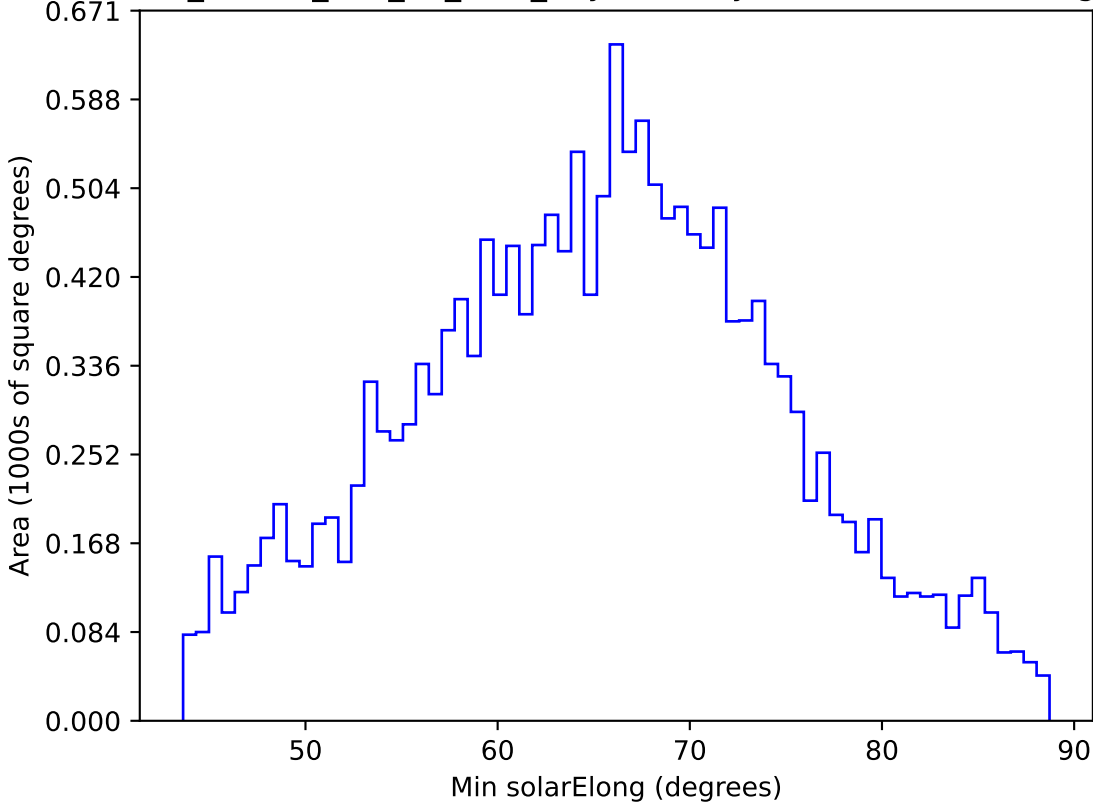
ddf_loaded_half_fl2_v3.4_10yrs WFD y band: Min solarElong
