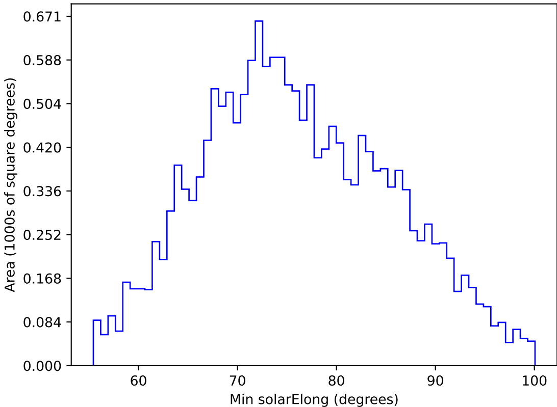
ddf_loaded_half_fl2_v3.4_10yrs WFD u band: Min solarElong
