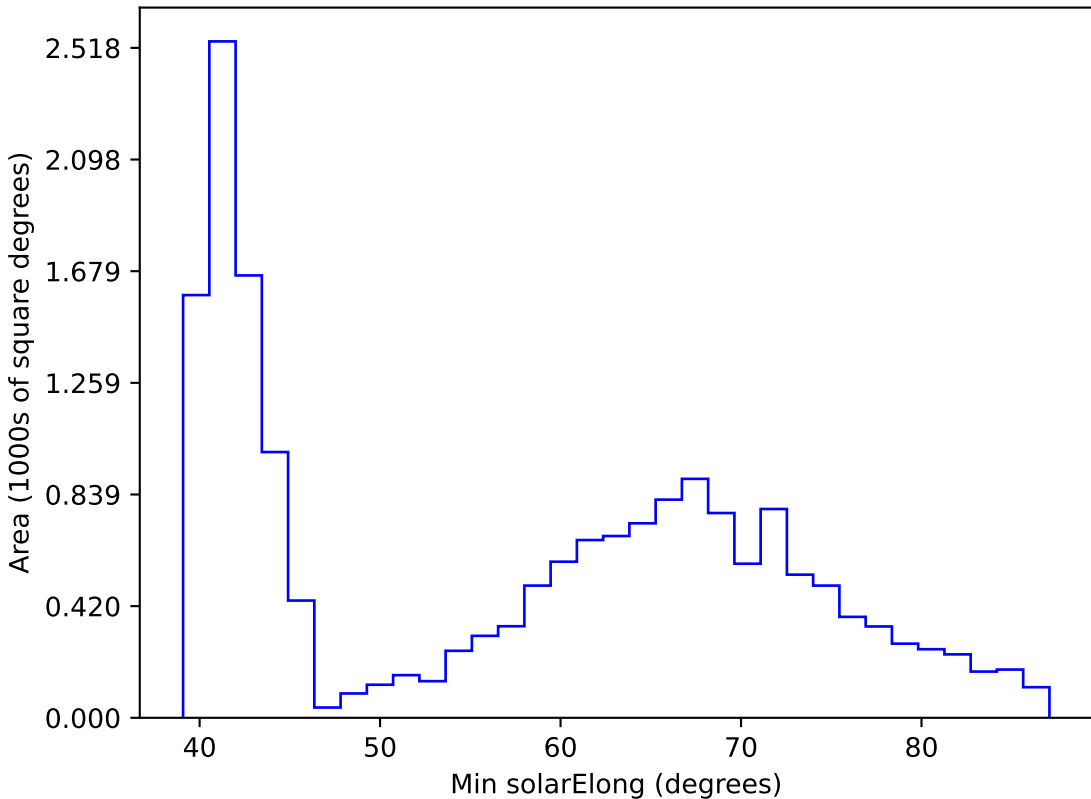
ddf_loaded_half_fl2_v3.4_10yrs WFD r band: Min solarElong
