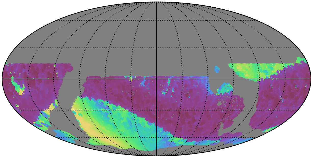
ddf_loaded_half_fl2_v3.4_10yrs WFD i band: Min solarElong
