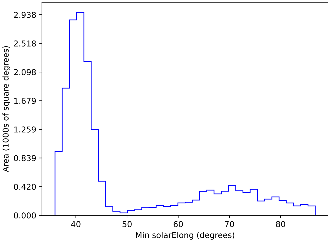
ddf_loaded_half_fl2_v3.4_10yrs WFD i band: Min solarElong
