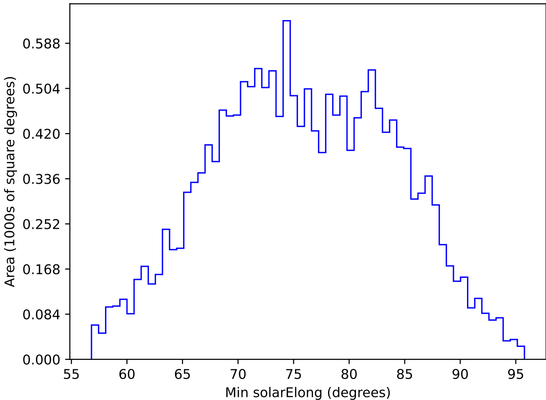
ddf_loaded_half_fl2_v3.4_10yrs WFD g band: Min solarElong
