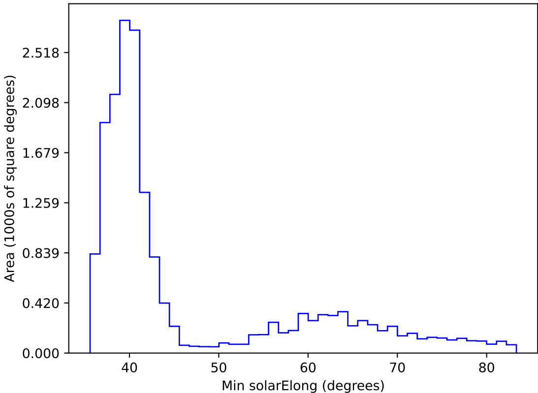
ddf_loaded_half_fl2_v3.4_10yrs WFD all bands: Min solarElong
