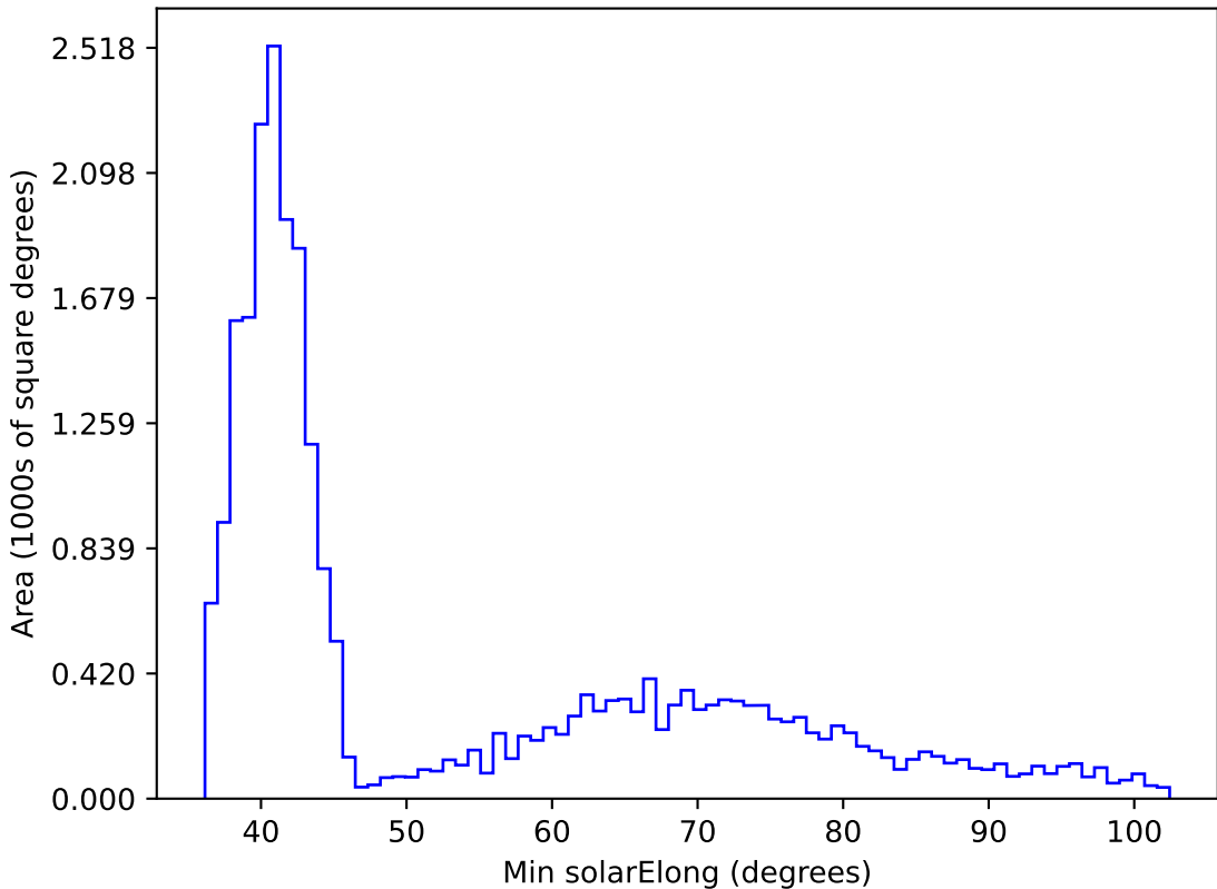
ddf_loaded_half_fl2_v3.4_10yrs All sky z band: Min solarElong
