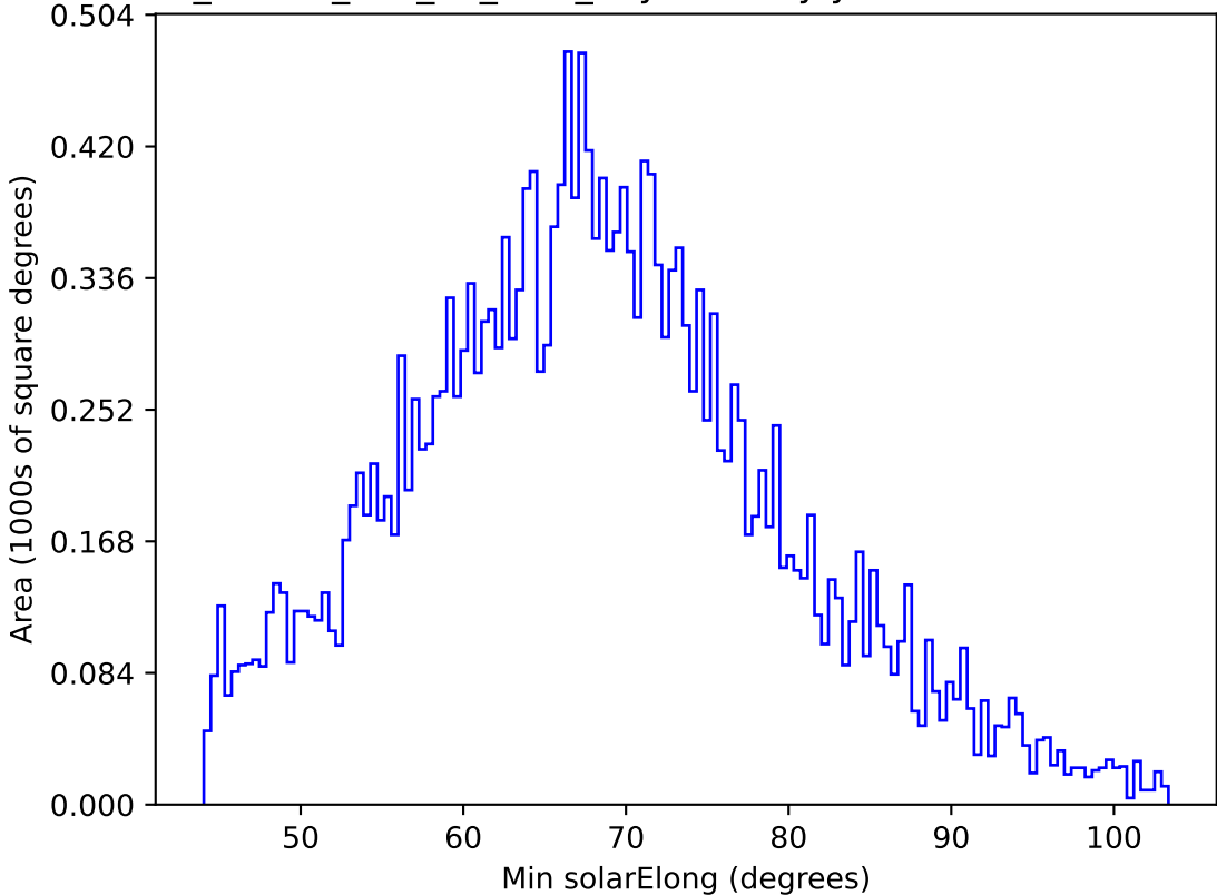
ddf_loaded_half_fl2_v3.4_10yrs All sky y band: Min solarElong
