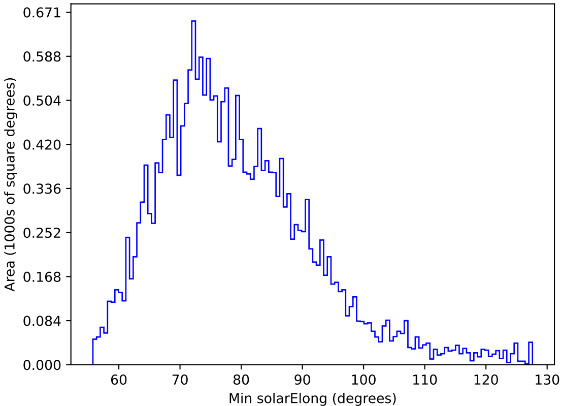
ddf_loaded_half_fl2_v3.4_10yrs All sky u band: Min solarElong
