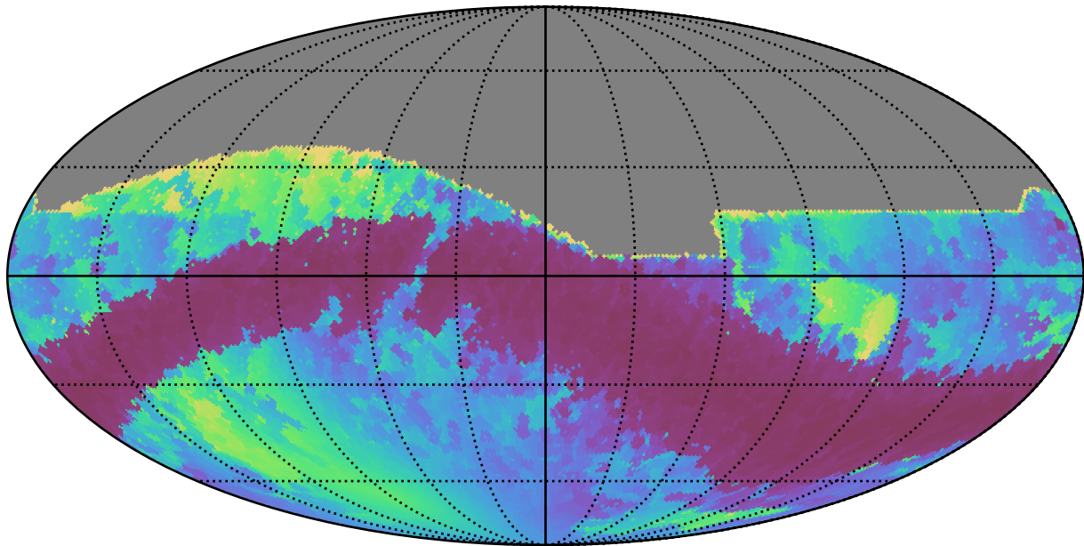
ddf_loaded_half_fi2_v3.4_10yrs All sky r band: Min solarElong
