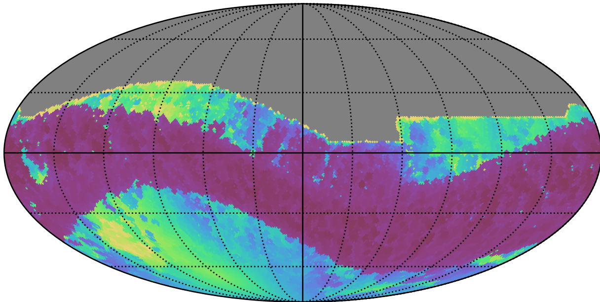
ddf_loaded_half_fl2_v3.4_10yrs All sky i band: Min solarElong
