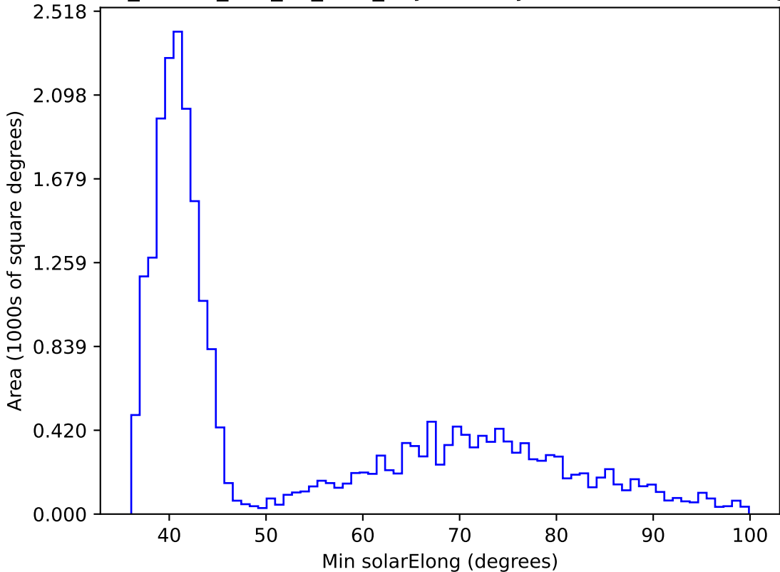
ddf_loaded_half_f12_v3.4_10yrs All sky i band: Min solarElong
